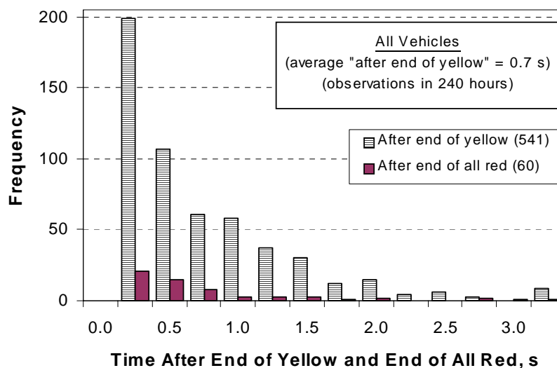
FIGURE 3 Frequency of red-light-running as a function of time into red.
