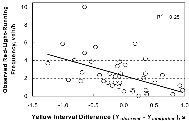
FIGURE 5 Red-light-running frequency as a function of yellow interval difference.
