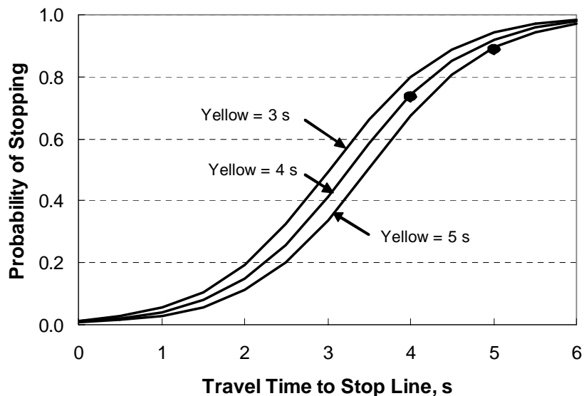
FIGURE 2 Probability of stopping as a function of travel time and yellow duration.
