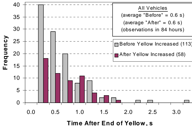
FIGURE 4 Effect of an increase in yellow interval duration on the frequency of red-light-running.
